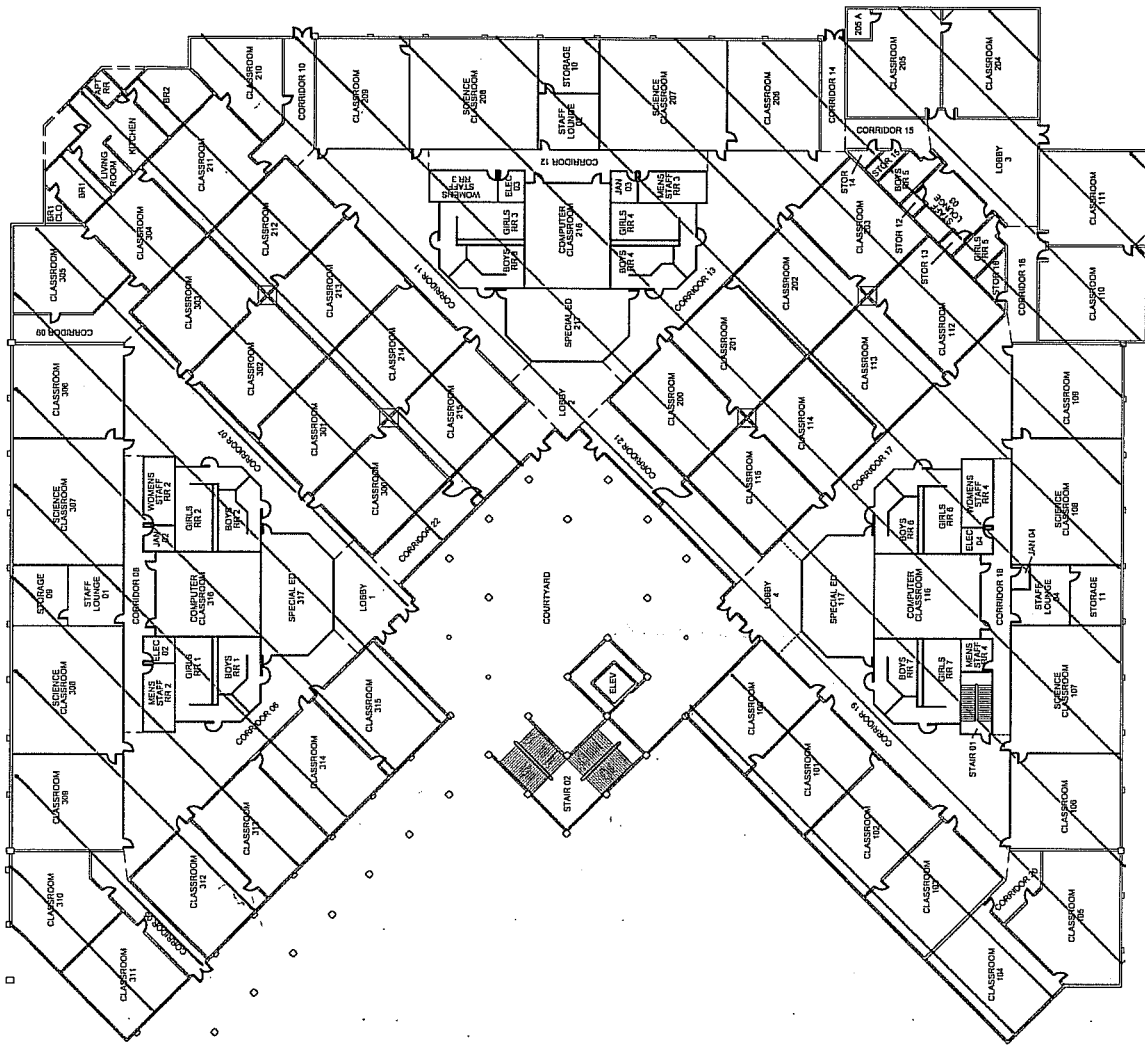
2ND FLOOR PLAN N.T.S.
