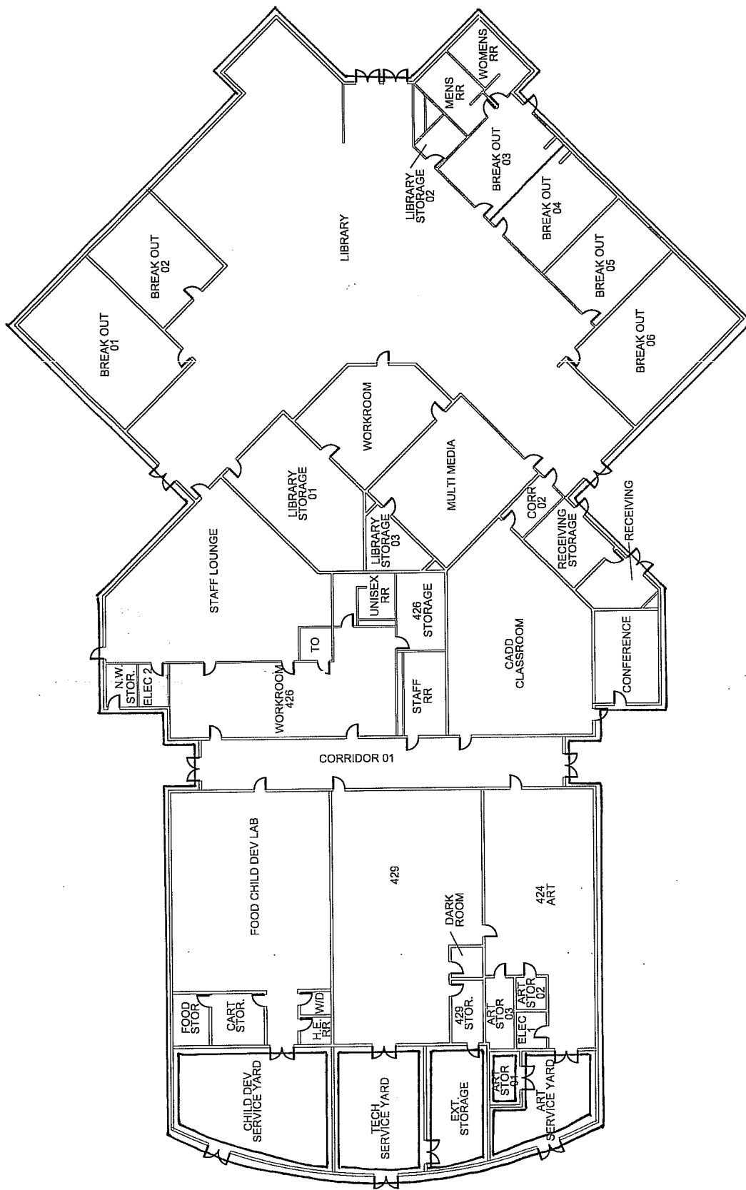
FLOOR PLAN N.T.S. NORTH
